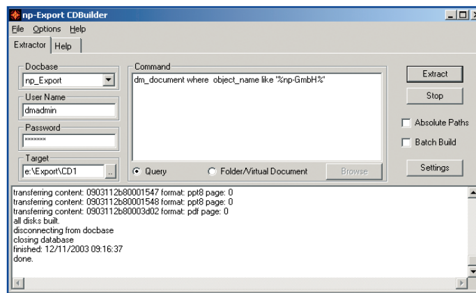
The Client of np-Export: the CDBuilder exports documents from the Documentum Docbase
