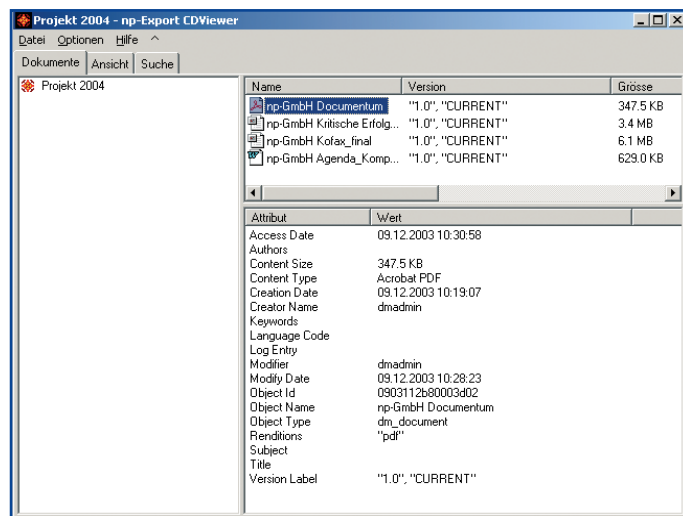
Viewing the CD: the user can use the CDViewer to inspect the documents without the Documentum Client
